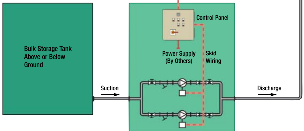
Midcom Transfer Pumpset with Integrated Electrical Control
